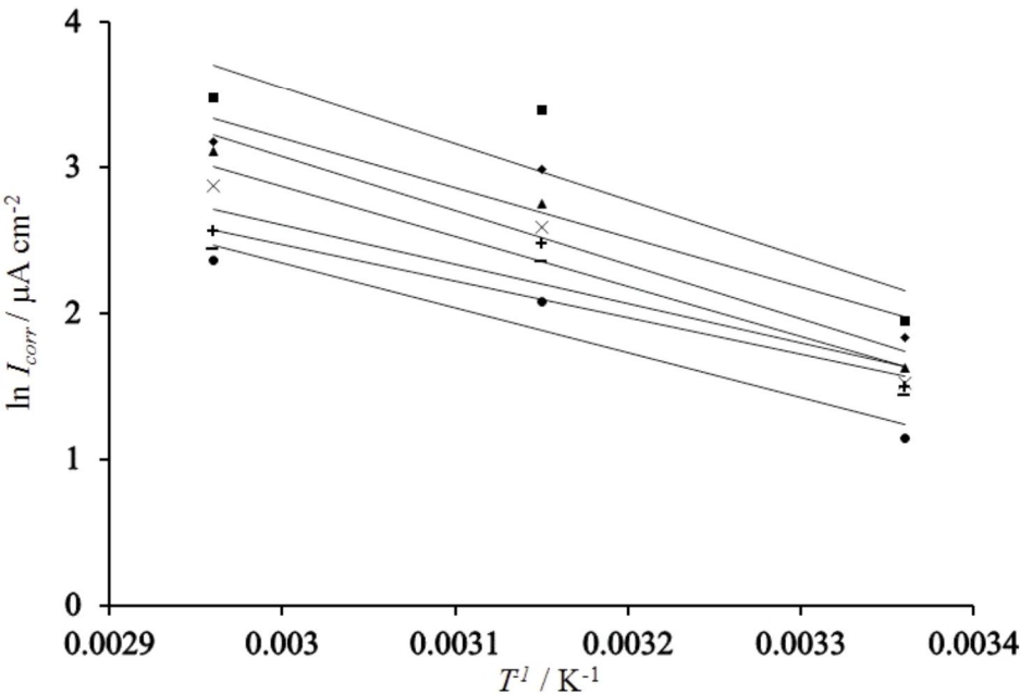
Fig. 5. Typical Arrhenius plots of \ln I_{\text{corr}} vs. 1/T for mild steel in alkaline 3% NaCl (pH=10) at different concentrations of inhibitor: □) Blank, ◇) 1 \times 10^{-6} , Δ) 3 \times 10^{-6} , ×) 5 \times 10^{-6} , +) 5 \times 10^{-5} , −) 3 \times 10^{-5} , ○) 7 \times 10^{-5} .
