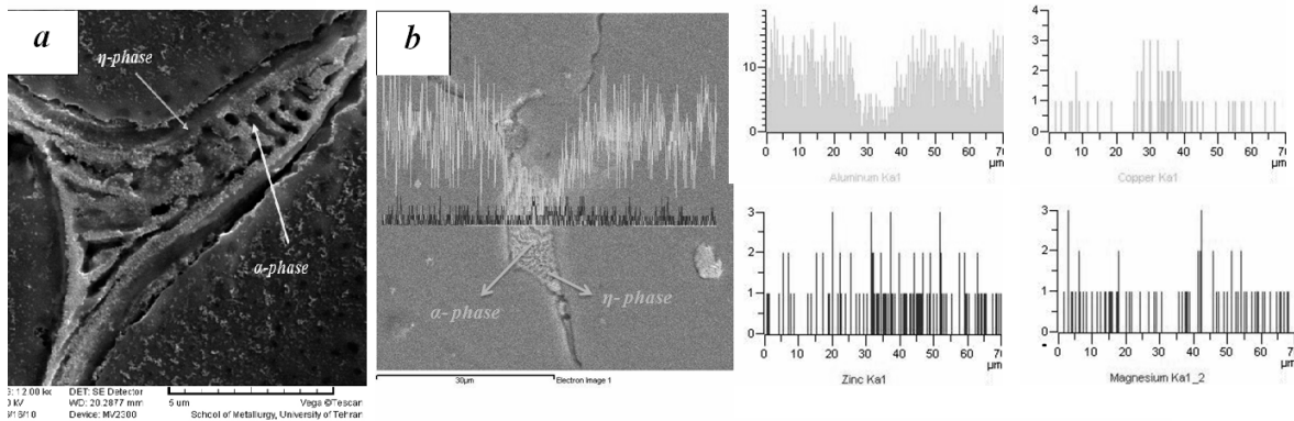
Fig. 4. (a) BSE image of the eutectic structure of as-cast sample (b) Results from line analysis in sample.
