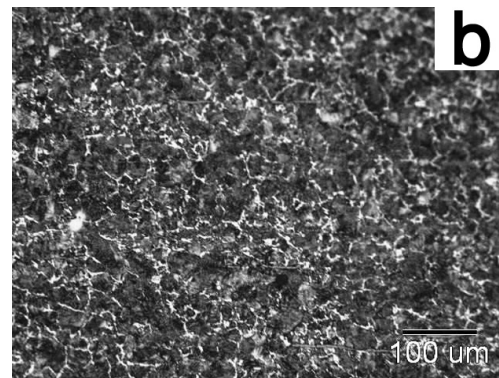
Fig. 5. The microstructure of HAZ, (a) near the base metal (50 mm distance from the weld center) and (b) near the fusion zone (30 mm distance from the weld center).
