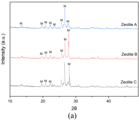
Fig. 2. a) XRD patterns of natural zeolite used in this study b) compounds found in natural zeolite used in this study
