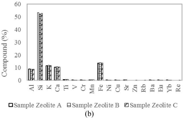
Fig. 2. a) XRD patterns of natural zeolite used in this study b) compounds found in natural zeolite used in this study
