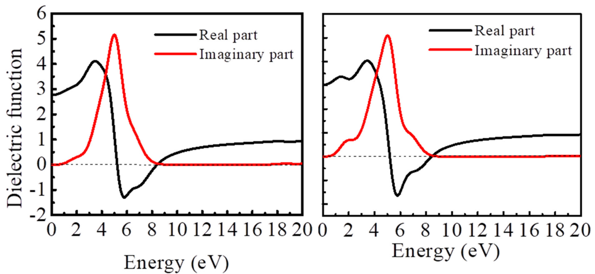
(a) \text{Sr}_{0.875}\text{Cr}_{0.125}\text{TiO}_3
