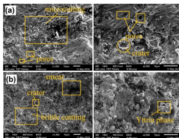
Fig. 8. Erosion mechanisms on WOKA-Y coating by the effect of (a) FA and (b) BA slurry at T = 180 min, C = 60\% (by wt.), \alpha = 0^\circ , and N = 1500 rpm
