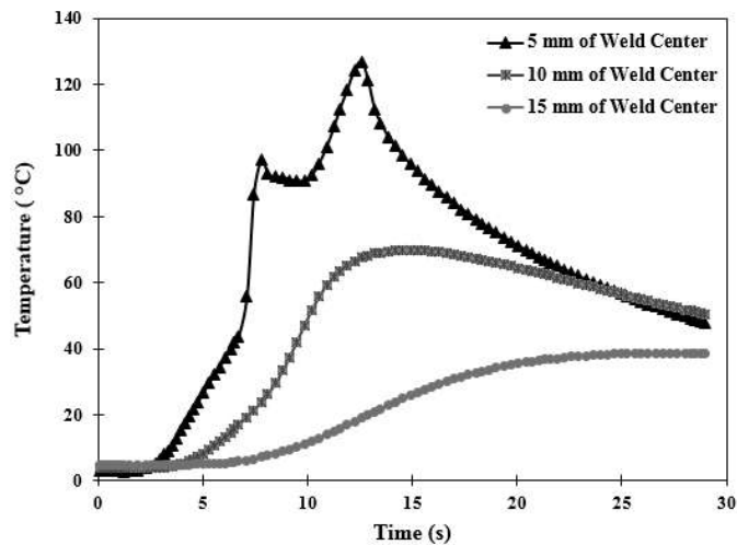
Fig. 7. Simulated top surface temperature distribution (1400 rpm–20 mm/min).
